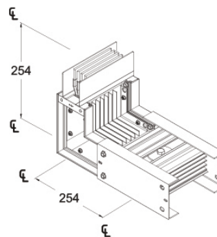
Edgewise Elbow
