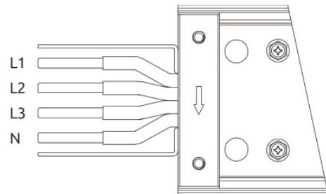
4. 3P3W + 100% Neutral + 50% Internal Ground
