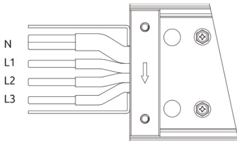
7. 3P3W + 200% Neutral + 50% Internal Ground
