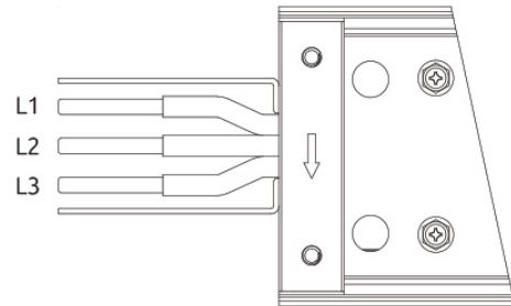
2. 3P3W + 50% Internal Ground
