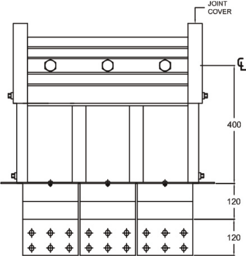
Case and Bars Three Bar Per Phase
