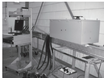
Thermal cycling test
