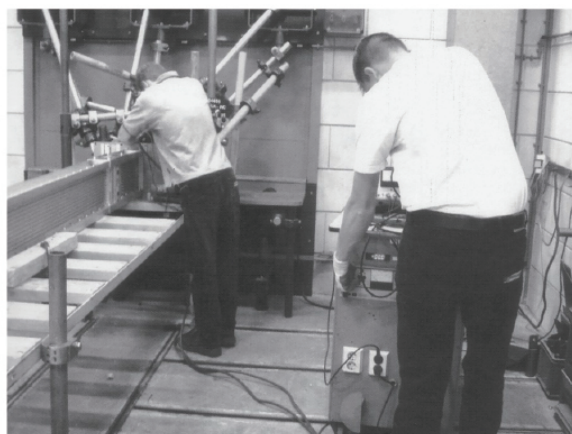
Thermal cycling test
