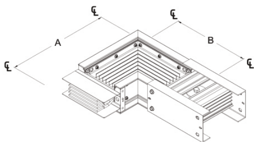
Flatwise Elbow
