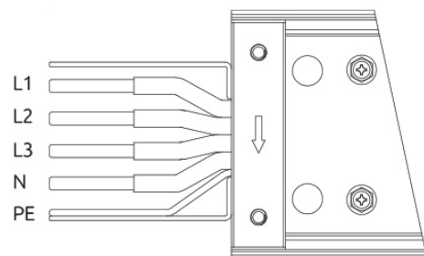
5. 3P3W + 100% Neutral + 100% Internal Ground
